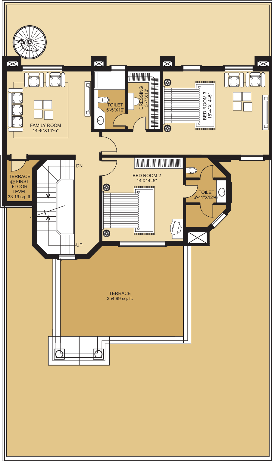
first floor
