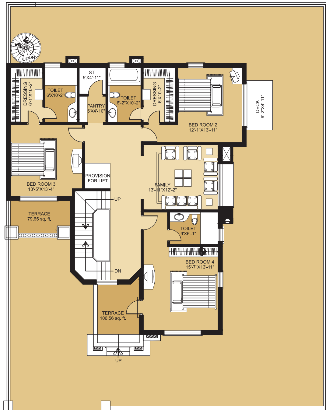
first floor
